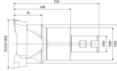
AKKO® ABHR-D120x160-W40-L210-CC12
