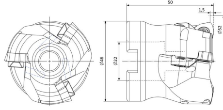
AKKO® AHFMC-JD1204-D052-A22-Z03-H
