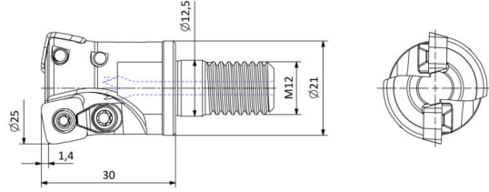
AKKO® AHFMC-SD09T3-D25-M12-L30-Z02-H
